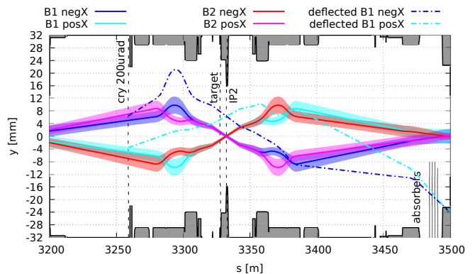
FIG. 2. The proposed layout of the ALICE-FT experiment. Both beams (B1 and B2) with their envelopes ( 7.3 \sigma ) are given with solid lines for both ALICE solenoid polarities ( posX and negX ). Deflected beams are given in dashed blue lines. The machine aperture is given in solid black lines. Vertical dashed lines mark the locations of crystals, target and IP2, respectively. The location of absorbers is marked in the right bottom corner.
