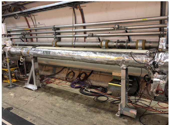
FIG. 3. Conditions inside the LHC tunnel at the proposed location for an installation of the crystal.
