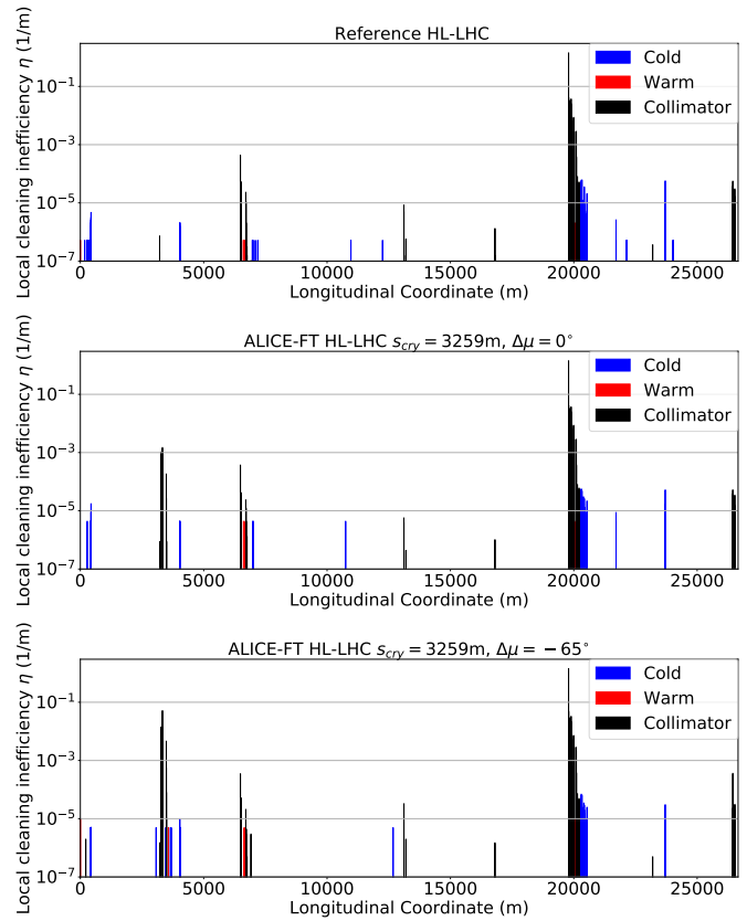
FIG. 4. Comparison of loss maps for the machine without (top) the ALICE-FT system, with the ALICE-FT system without the optics optimisation (middle) and with the ALICE-FT system with the optics optimisation (bottom). The local cleaning inefficiency (vertical axis) is a measure of the number of protons not intercepted by the collimation system and impacting the machine aperture. The simulation limit of 1 proton lost in the machine aperture corresponds to 5 \cdot 10^{-7} \text{m}^{-1} in a 10 cm longitudinal bin. No abnormal loss spikes are present in the loss maps.
