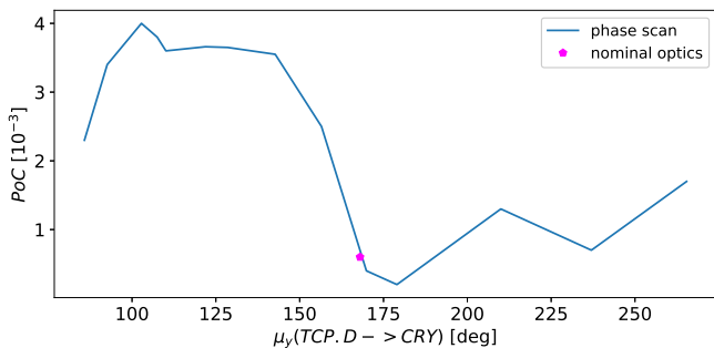
FIG. 5. The dependence of the fraction of the number of protons impacting the crystal over the number of protons impacting the primary collimator (PoC) on the betatron phase from the primary vertical collimator in IR7 (TCP.D) to the IR2 crystal (CRY). Crystal retraction is 7.9 \sigma .
